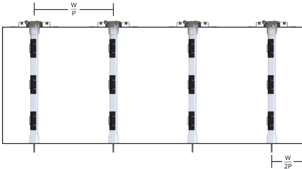
Probe Spacing
